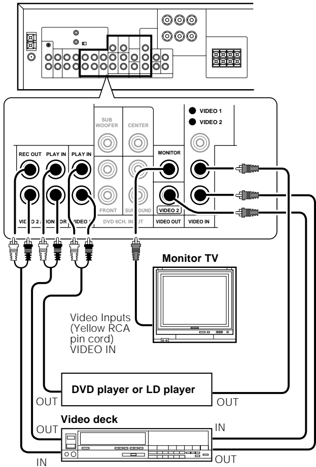
Audio inputs and outputs (Red and white RCA pin cords)
